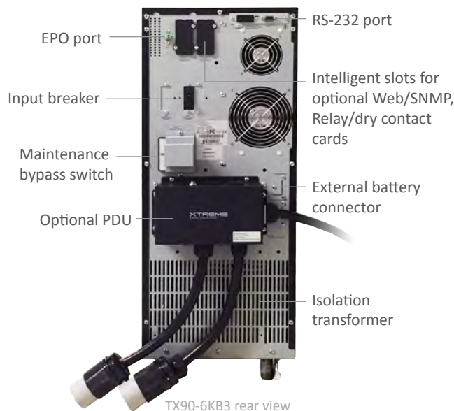
TX90-6KB3 rear view
